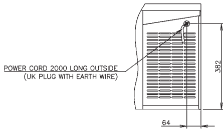
VIEW A (1/10)
