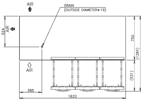
VIEW A (1/10)
